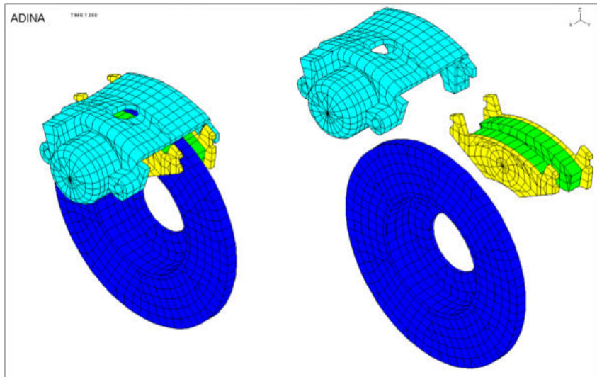
Figure 5 FEM-model of breaking system N = 67986
