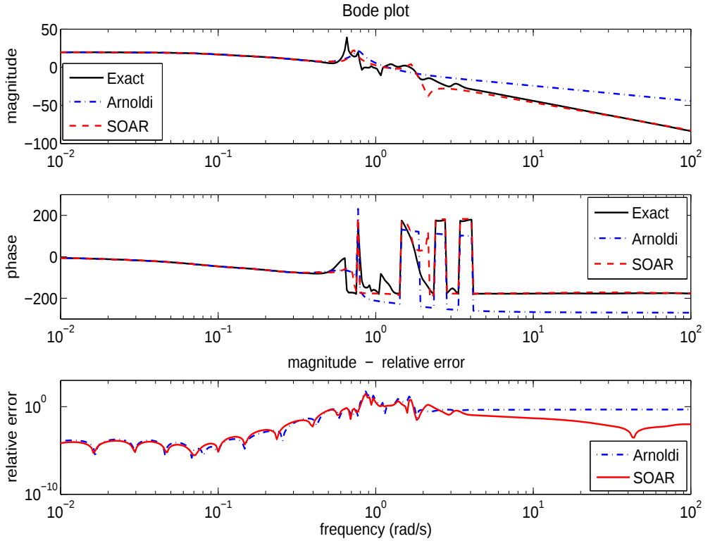
Figure 8 Bode plot SOAR/Arnoldi, n = 10 , expansion point s_0 = 0.1
