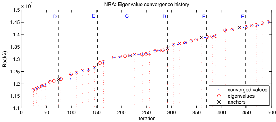
Fig. 9 Eigenvalue convergence history throughout first 500 iterations of NRA while computing eigenvalues in (11748, 16820] of the gyroscopic wheel problem.
