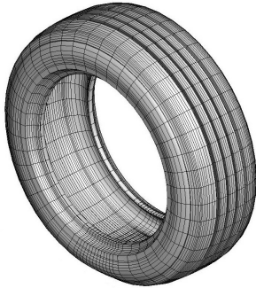
Fig. 12 Continental AG 205/55R16-91H tire.
