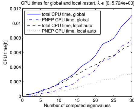
Fig. 5 Global versus local restart with automatic balancing - zoom into the lower end of the spectrum in Figure 3. We observe that the balancing effectively restores the superior performance of the local restart over the global restart also in the initial phase.
