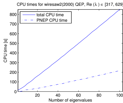
Fig. 11 CPU time of NRA for computation of eigenvalues with real part in [317, 629] of the NLEVP "wiresaw2" problem of dimension 2000.
