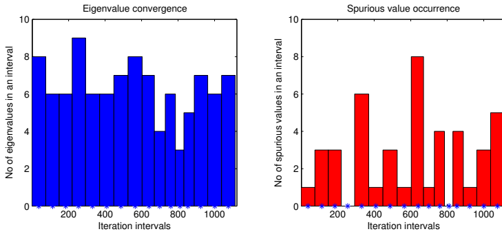
Fig. 8 Histogram of (a) eigenvalue convergence, (b) spurious value occurrence per interval between consecutive restarts in one run of computation of eigenvalues in (11748, 16820] of the gyroscopic wheel problem.
