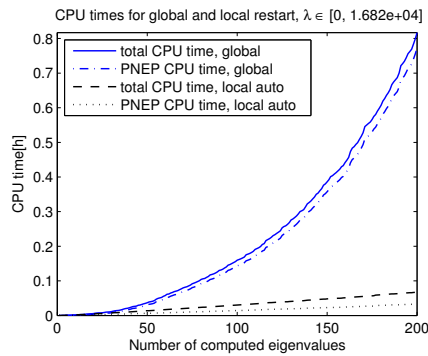
Fig. 3 Global versus local restart with automatic balancing for first 200 eigenvalues of the gyroscopic wheel problem.
