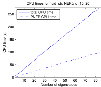
Fig. 15 CPU time of NRA for computation of eigenvalues in [10, 20] of the rational fluid structure interaction problem of dimension 36040.
