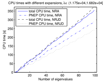
Fig. 7 CPU time of NRA and NRJD for computation of eigenvalues in (\lambda_{100} = 11748, 16820] of the gyroscopic wheel problem without automatic balancing.
