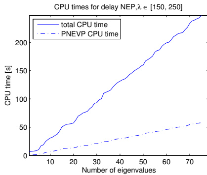
Fig. 14 CPU time of NRA for computation of eigenvalues in [150, 250] of the exponential delay problem of dimension 39601.
