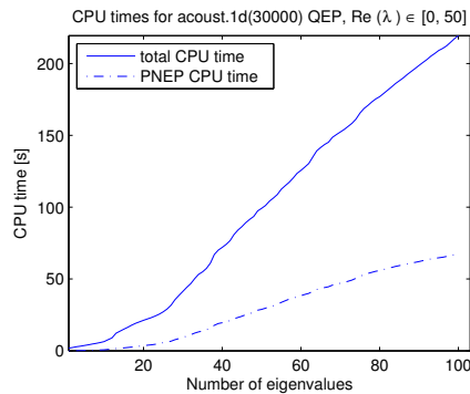
Fig. 17 CPU time of NRA for computation of eigenvalues with real part in [0, 50] of the NLEVP quadratic "acoustic wave 1d" problem of dimension 30000.
