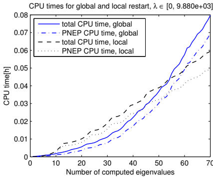
Fig. 4 Global versus local restart - zoom into the lower end of the spectrum in Figure 2. When computing the eigenvalues at the beginning of the spectrum in the initial phase the global restart can outperform the local restart with fixed search subspace dimension limit.
