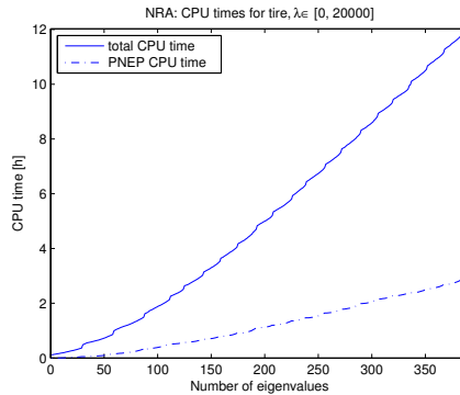
Fig. 13 CPU time for NRA for eigenvalues in [0, 20000] of the gyroscopic tire 205/55R16-91H problem.
