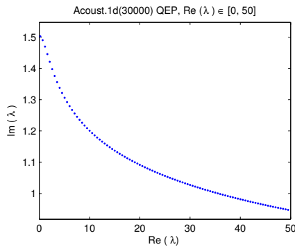
Fig. 16 Eigenvalues with the real part in [0, 50] of the NLEVP quadratic "acoustic wave 1d" eigenvalue problem of dimension 30000.
