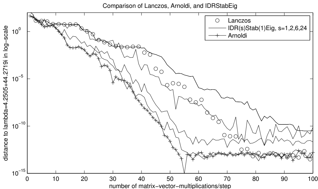
Figure 2: Comparison of Lanczos’s method, Sonneveld methods for varying s ( s = k! for k = 1, \dots, 4 ), and Arnoldi’s method. The starting vectors have been chosen such that Lanczos’s method is mathematically equivalent with IDR(1).
