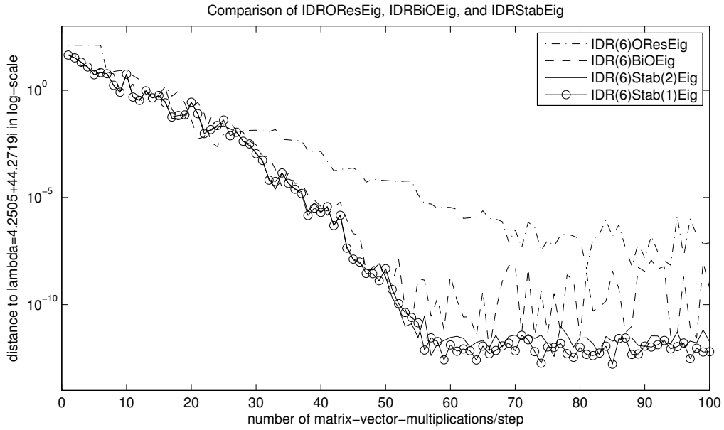
Figure 1: Comparison of the eigenvalue approximation behaviour of IDR(6)ORes, IDR(6)BiO, IDR(6)STAB(2) and IDR(6)STAB(1).
