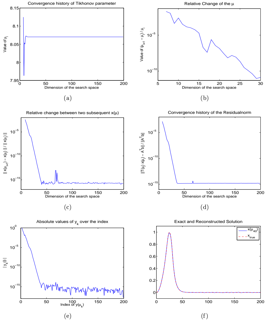
Figure 2: Convergence histories for Example 4.1.
