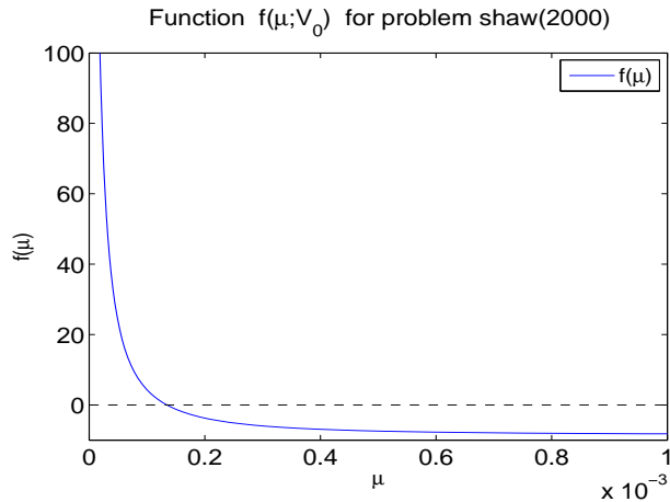
Figure 1: Plot of a typical function f(\mu) .
