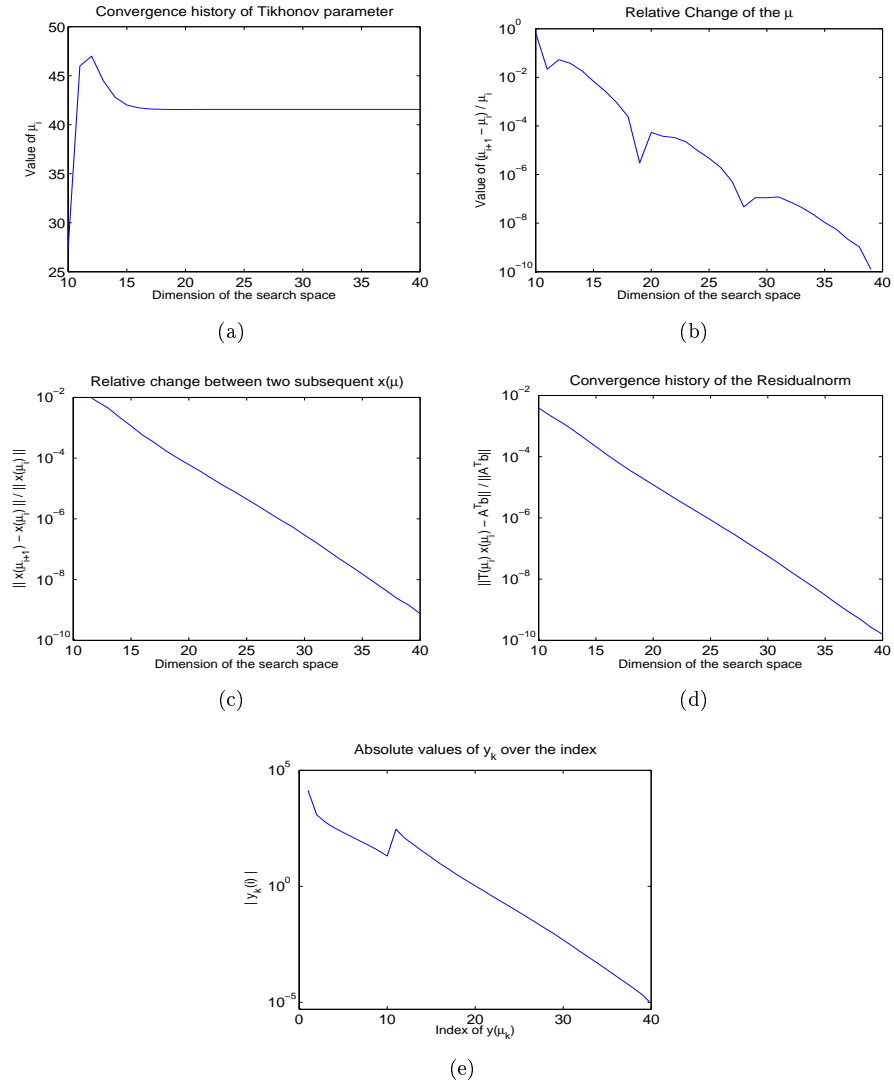
Figure 3: Convergence histories for the restoration of Danny using the regularization matrix L_{1,2D} .
