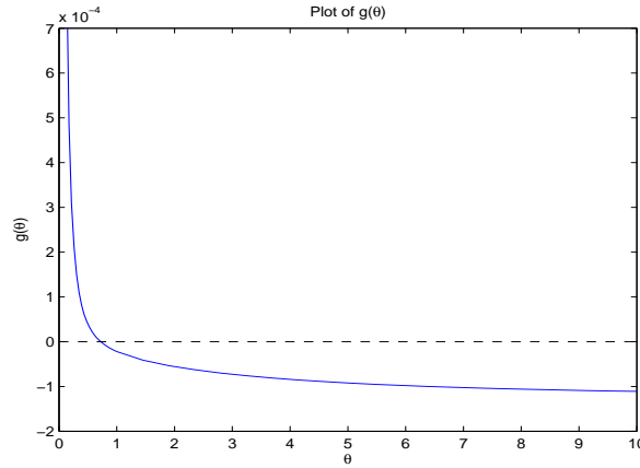
FIG. 3.1. Plot of a typical function g(\theta)
