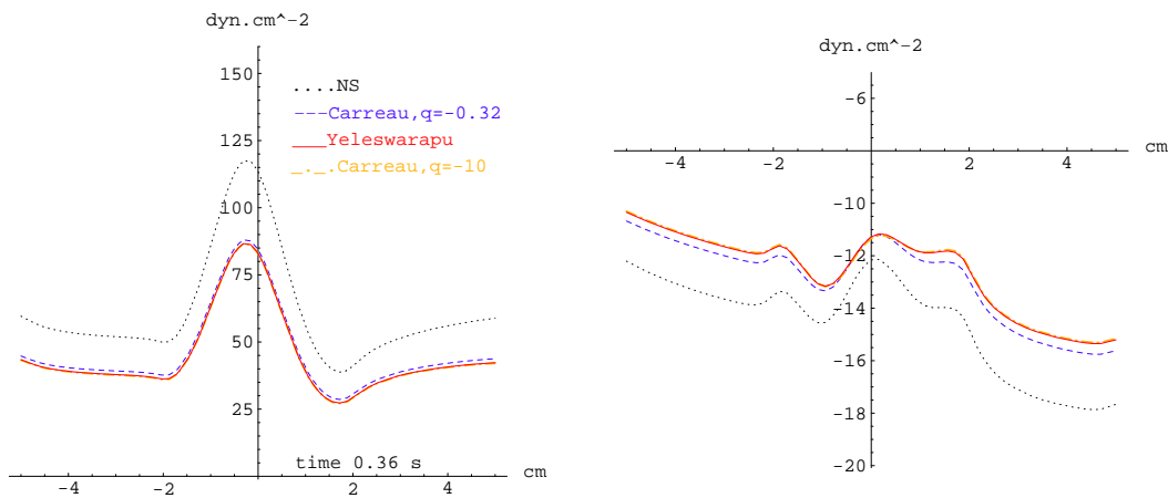
Figure 2. WSS : the Newtonian (NS), the Yeleswarapu viscosity function and the Carreau models
