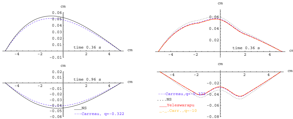
Figure 1. Wall deformation, left: the Newtonian (NS) and the Carreau models in the straight channel; right: the Newtonian (NS), the Yeleswarapu viscosity and the Carreau models in the stenosed channel
