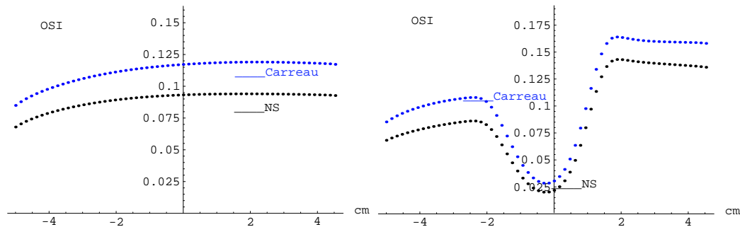
Figure 3. OSI indices computed using the Newtonian (NS) and the Carreau models with q = -0.322 in the straight channel (left) and in the stenosed channel (right)
